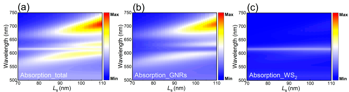
Figure 6. (a) Two-dimensional absorption spectrum calculated for a T-shaped GNR dimer with variant length of the short GNR placed on a WS 2 monolayer. (b) Two-dimensional absorption spectrum calculated for a T-shaped GNR dimer with variant length of the short GNR. (c) Two-dimensional absorption spectrum obtained by subtracting the spectrum shown in (b) from that shown in (a).
