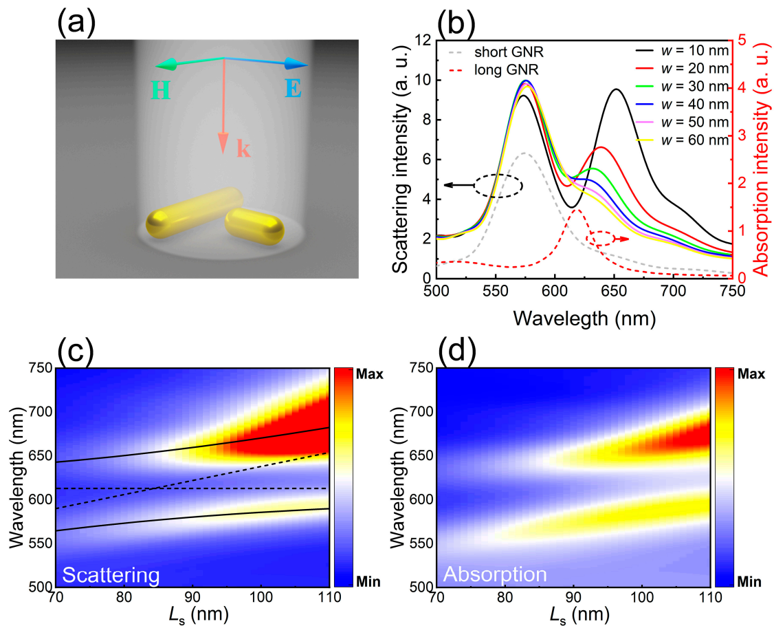
Figure 2. Strong coupling between the dipole and quadrupole modes excited in a T-shaped GNR dimer. (a) Schematic showing the T-shaped GNR dimer composed of a long and a short GNR and the wavevector and the electric/magnetic field of the plane wave used to excite the GNR dimer. (b) Scattering spectra calculated for GNR dimers with different gap widths ( w ). The scattering spectrum of the isolated short GNR (gray dashed curve) and the absorption spectrum of the isolated long GNR (red dashed curve) are also provided. (c) Two-dimensional scattering spectra calculated for GNR dimers composed of short GNRs with different lengths. The fitting results based on Equation (1) are also provided. (d) Two-dimensional absorption spectra calculated for GNR dimers composed of short GNRs with different lengths.
