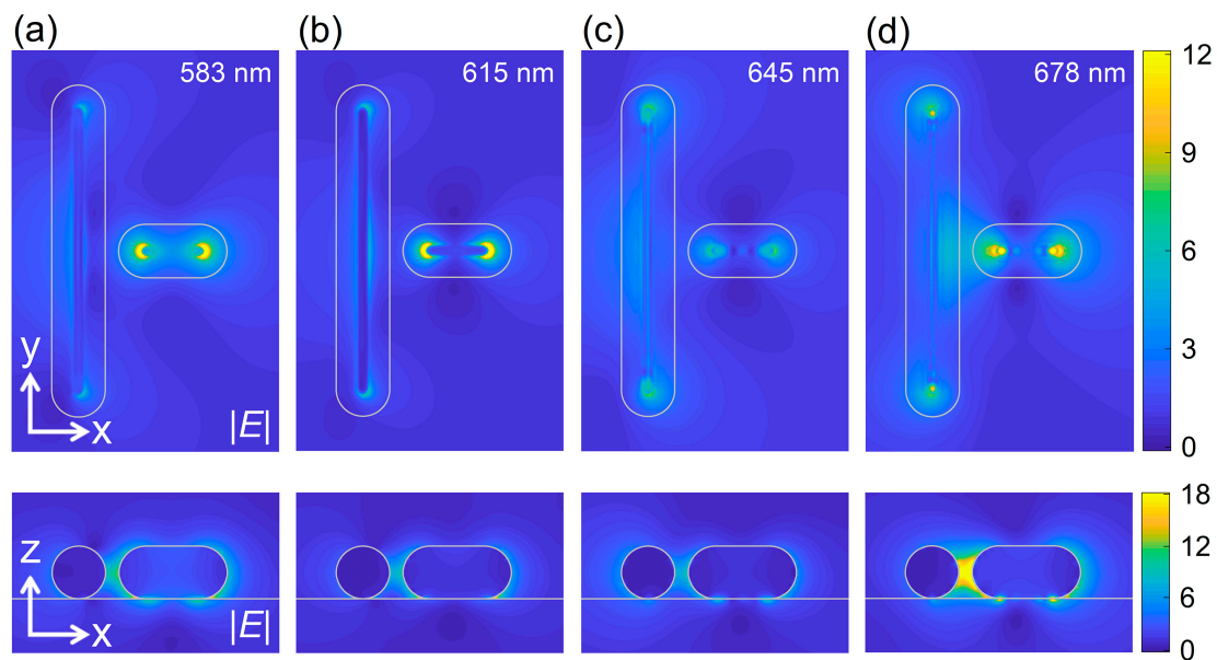
Figure 7. Electric field distributions in the XY (upper panel) and XZ planes (lower panel) calculated for the T-shaped GNR dimer placed on a WS 2 monolayer with L_l = 248 nm, L_s = 81 nm and w = 10 nm at different wavelengths. (a) \lambda = 583 nm, (b) \lambda = 615 nm, (c) \lambda = 645 nm and (d) \lambda = 678 nm.
