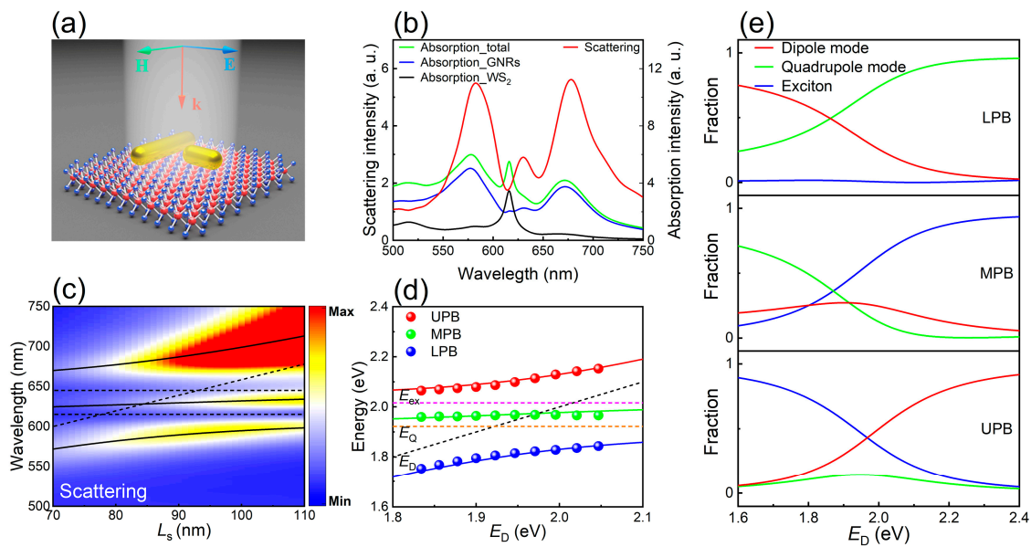
Figure 5. Strong dipole–quadrupole–exciton coupling realized in a T-shaped GNR dimer placed on a monolayer WS 2 . (a) Schematic showing a T-shaped GNR dimer placed on a monolayer WS 2 and excited by a plane wave. (b) Scattering spectrum calculated for the GNR dimer placed on a WS 2 monolayer with L_l = 248 nm, L_s = 81 nm and w = 10 nm. The absorption spectra of the long and short GNRs only and the absorption spectrum of the monolayer WS 2 are also provided. (c) Two-dimensional scattering spectra calculated for GNR dimers composed of short GNRs with different lengths. (d) The red, green and blue circles represent the upper, middle and lower polariton branch (UPB, MPB and LPB) resonance energies extracted from the scattering spectrum of T-shaped GNR dimer placed on a WS 2 monolayer hybrid structure. The red, green and blue solid lines represent the resonance energies of UPB, MPB and LPB fitted by Hamiltonian analysis Equation (3). The black, orange and pink dashed lines represent dipole, quadrupole and exciton resonances, respectively. (e) Hopfield coefficients for dipole, quadrupole and exciton modes contributions to UPB, MPB and LPB as a function of dipole resonance.
