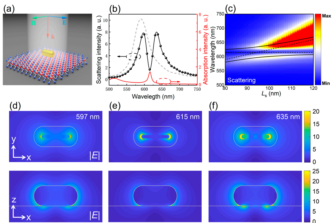
Figure 4. Strong coupling between the dipole mode in a single GNR and the excitons in a monolayer WS 2 . (a) Schematic showing the excitation of a single GNR placed on a monolayer WS 2 by using plane wave. (b) Scattering spectrum (black solid curve) calculated for a GNR resonant with the exciton resonance of the monolayer WS 2 . Additionally, shown are the scattering spectrum of the GNR in the absence of the monolayer WS 2 (dashed curve) and the absorption spectrum of the monolayer WS 2 (red solid curve). (c) Two-dimensional scattering spectra calculated for GNRs with different lengths. The fitting results based on Equation (2) are also provided. (d)–(f) Electric field distributions in the XY plane (upper panel) and XZ plane (lower panel) calculated for the GNR with L_s = 94 nm at different wavelengths of \lambda = 597 , 615 and 635 nm, respectively.
