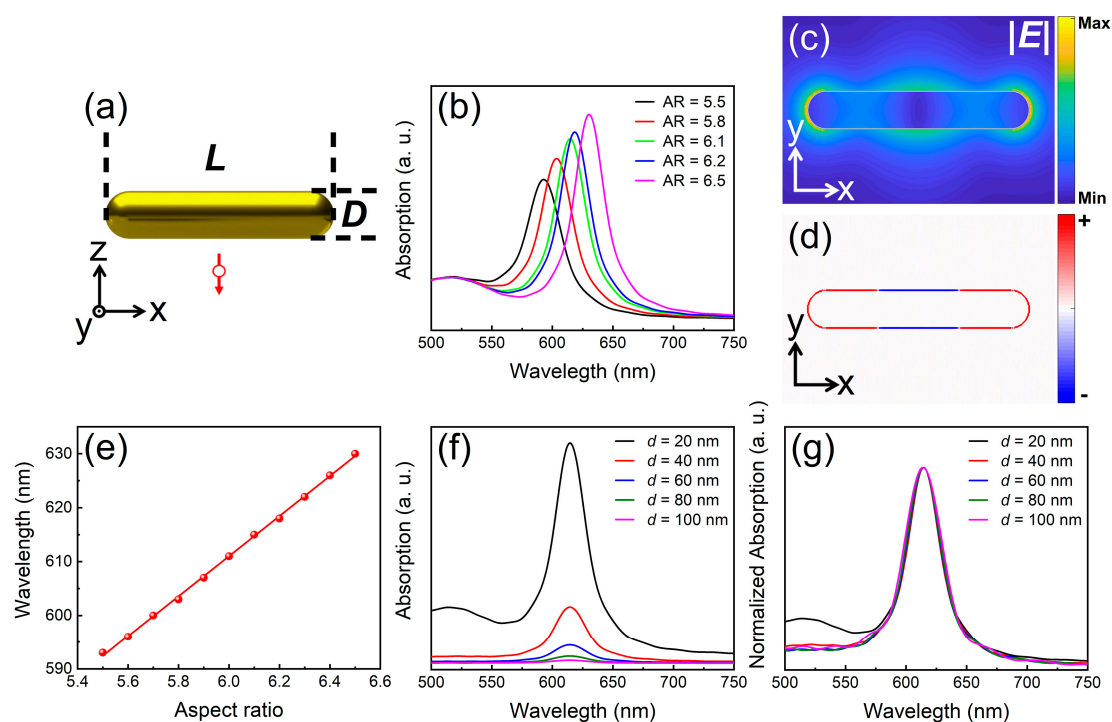
Figure 1. Excitation of the quadrupole mode in a GNR by using a dipole source. (a) Schematic showing a GNR with a length of L and a diameter D and a dipole source placed nearby. (b) Absorption spectra calculated for GNRs with different aspect ratios. Electric field (c) and surface charge (d) distributions calculated for a GNR with AR = 6.1 at \lambda = 615 nm. (e) Dependence of the resonance wavelength on the aspect ratio of the GNR. (f) Absorption spectra calculated for the long GNR (AR = 6.1), which is excited by a dipole source placed at different distances ( d ). (g) Normalized absorption spectra of the long GNR shown in (f).
