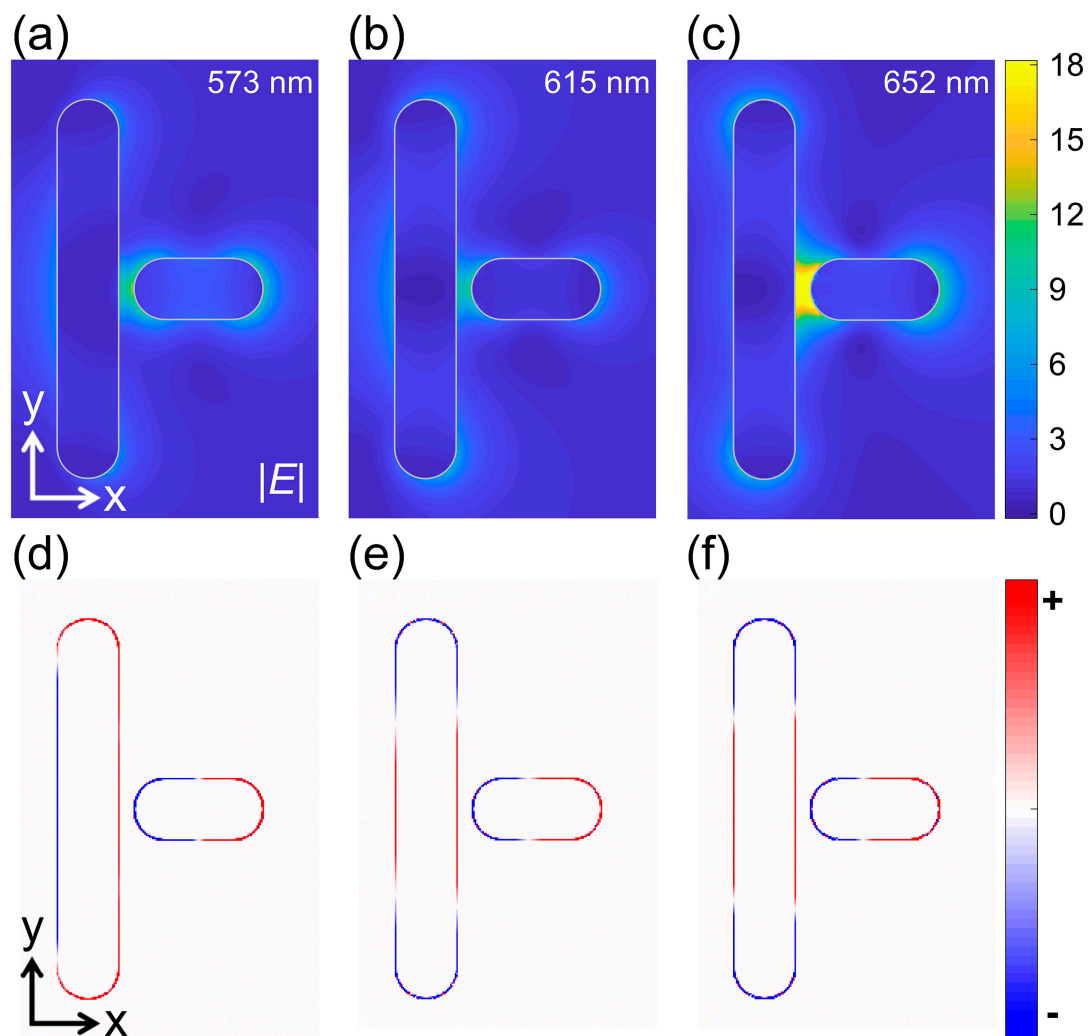
Figure 3. Electric field (upper panel) and surface charge (lower panel) distributions calculated for the T-shaped GNR with L_l = 248 nm, L_s = 84 nm and w = 10 nm at different wavelengths. (a,d) \lambda = 573 nm, (b,e) \lambda = 615 nm, (c,f) \lambda = 652 nm.
