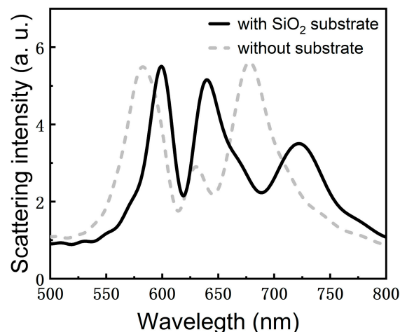
Figure 8. Scattering spectrum calculated for a GNR dimer placed on a SiO 2 substrate with an embedded WS 2 monolayer (black solid curve). The scattering spectrum of the hybrid structure in the absence of the substrate is also provided for comparison (dashed curve).
