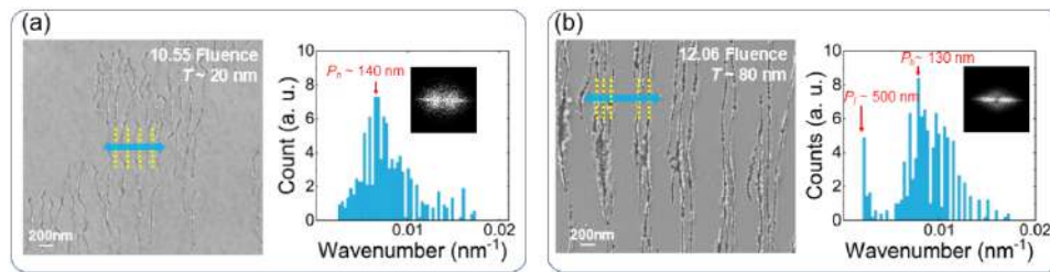
Fig. 2. (a) The SEM image and the corresponding Fourier transformation spectrum and image of the nanoripple form on a multilayer \text{WS}_2 film with a thickness of T \sim 20 \text{ nm} . (b) The SEM image and the corresponding Fourier transformation spectrum and image of the nanoripple form on a multilayer \text{WS}_2 film with a thickness of T \sim 80 \text{ nm} . In each image, the yellow dashed line represents the orientation of the nanoripple, and the blue arrow indicates the writing laser polarization orientation.
