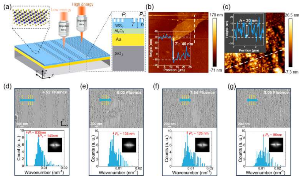
Fig. 1. (a) Schematic of writing process and structure of low- and high-spatial-frequency nanoripples on the surface of multilayer WS 2 placed on an Al 2 O 3 /Au/SiO 2 substrate by using focused femtosecond laser pulses at 800 nm. (b) The AFM image of the uniform multilayer WS 2 film, the height profile along the white dashed line is shown in the inset indicating a film thickness of T \sim 40 nm. (c) The AFM image of a typical high-spatial-frequency nanoripple, the height profile along the white dashed line is shown in the inset indicating a nanoripple depth of h \sim 20 nm. (d-e) The SEM images of nanoripples induced by laser irradiation at energy densities of 4.52, 6.03, 7.54, and 9.05 mJ/cm 2 , respectively (upper panels). In each image, the yellow dashed line represents the orientation of the nanoripple, and the blue arrow indicates the writing laser polarization direction. The lower panels and insets show the corresponding Fourier transformation spectra and images, revealing the period and orientation of the nanoripples.
