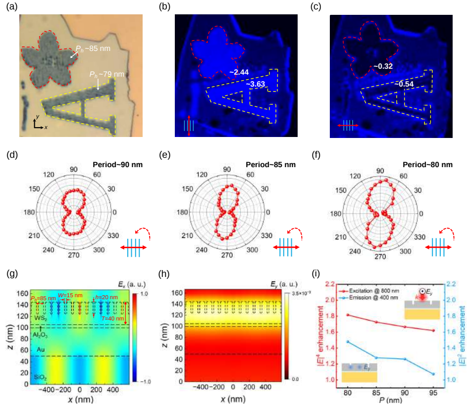
Fig. 4. Polarization-dependent second harmonic waves produced by the uniform WS 2 film and the nanoripple. (a) Bright-field image of nanoripple patterns fabricated on a WS 2 film. The periods of the nanoripples in the regions of “flower” and “letter A” are \sim 85 nm and \sim 79 nm, respectively. (b) and (c) show SHG scanning images excited by low-fluence femtosecond laser pulses at the wavelength of 800 nm, where y-polarized and x-polarized light are used, respectively. The red arrow and blue lines show the polarization of the scanning laser and the orientation of nanoripples, respectively. The SHG enhancement and reduction factors of nanoripples compared to the uniform WS 2 film are also displayed in the figures. (d)-(f) show the polarization-dependent amplitude of the second harmonic wave in the nanoripples with different periods. The polarization angle of the incident laser is changed in steps of 10°. (g) Simulated E_x distribution in the x-z plane excited by an x-polarized (perpendicular to the nanoripple) plane wave at 800 nm. (h) Simulated E_y distribution in the x-z plane excited by a y-polarized (parallel to the nanoripple) plane wave at 800 nm. (i) The enhancement factors of y-polarized light at excitation (800 nm) and emission (400 nm) wavelengths produced by the nanoripple.
