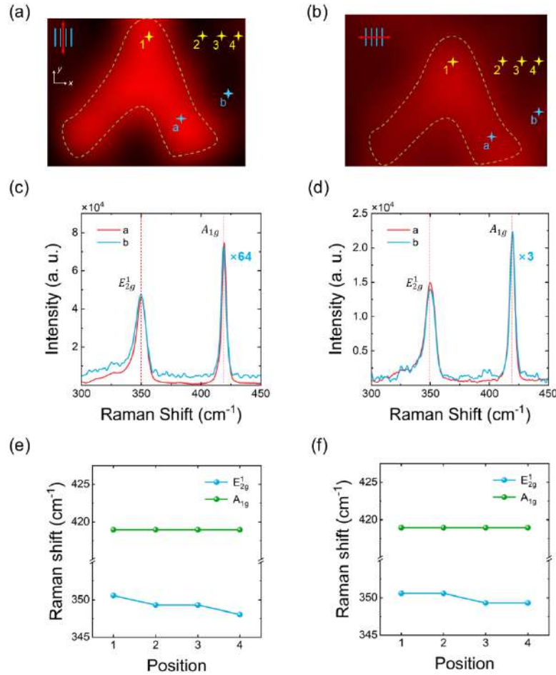
Fig. 5. Polarization-dependent Raman signals of the nanoripple with a period of \sim 85 nm. (a) Raman scanning image of the WS 2 nanoripple at 350\text{ cm}^{-1} ( E_{2g}^1 mode) with y-polarized laser excitation. The blue lines indicate the orientation of the nanoripple, and the red arrow indicates the polarization direction of the scanning laser. (b) Raman scanning image of a WS 2 nanoripple at E_{2g}^1 mode with x-polarized laser excitation. (c) and (d) show the Raman spectra of the nanoripple (at point a) and the WS 2 thin film (at point b) under y- and x-polarized excitation, respectively. The blue curves in (c) and (d) are magnified by factors of 64 and 3, respectively, to facilitate direct comparison with the red curve data. (e) and (f) show the Raman shift extracted from four different locations (points 1, 2, 3, and 4) in (a) and (b), respectively.
