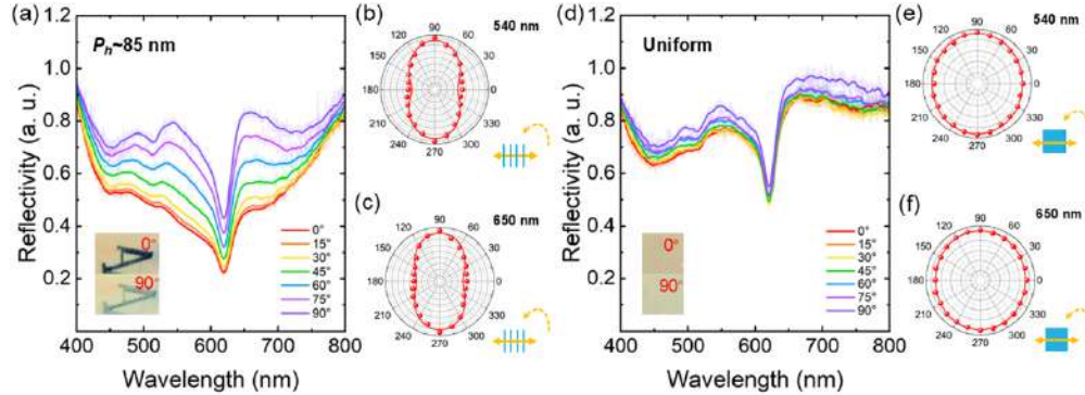
Fig. 3. Polarization-dependent reflectivity of the nanoripple. (a) Reflectivity spectra of the WS 2 nanoripple under illumination with white light at different polarization angles. The insets are bright-field images of the sample. The polarization characteristic of the WS 2 nanoripple at the wavelengths of (b) 540 nm, and (c) 650 nm are measured with the polarization angle varying from 0° to 360°. The inset shows the polarization (yellow arrow) of the probe light and the orientation of the nanoripple (blue lines). (d) Reflectivity spectra of the uniform WS 2 film under illumination with white light at different polarization angles. The polarization characteristic of the uniform WS 2 film at the wavelengths of (e) 540 nm, and (f) 650 nm are measured with the polarization angle varying from 0° to 360°.
